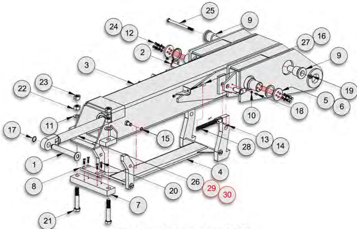
OUTER TUBE SUB-ASSEMBLY
