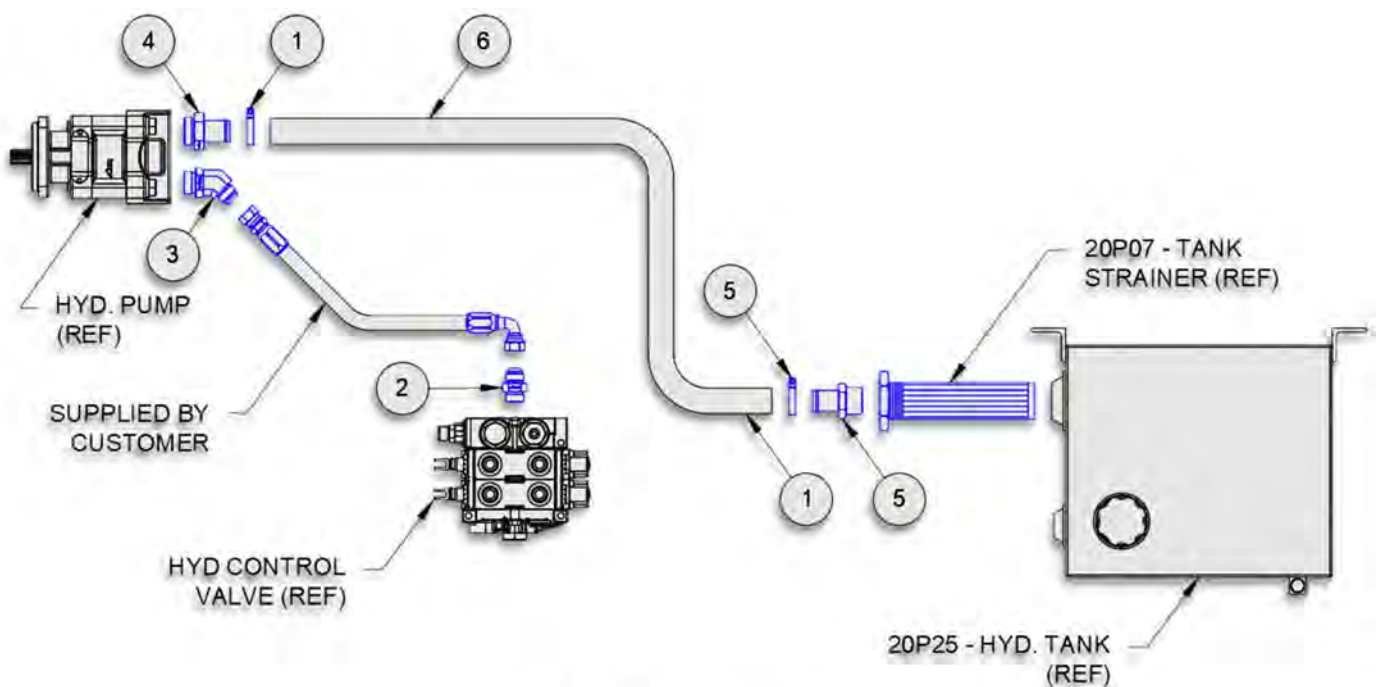
PUMP CIRCUIT
