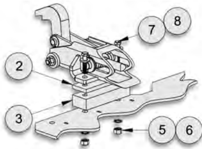
HYD BODY LOCK MOUNTING DETAIL
